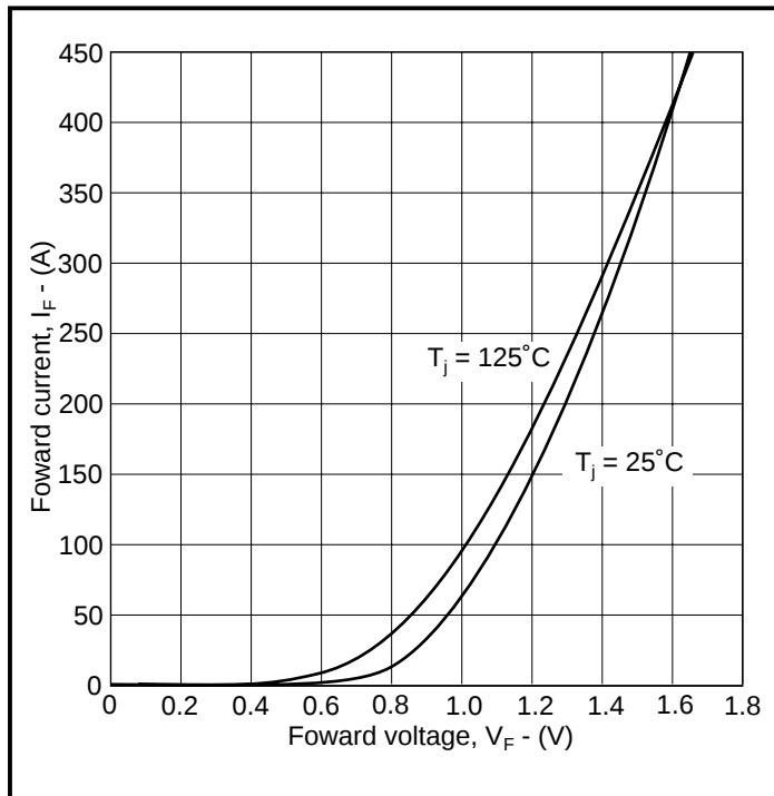
Fig.12 Diode typical forward characteristics
