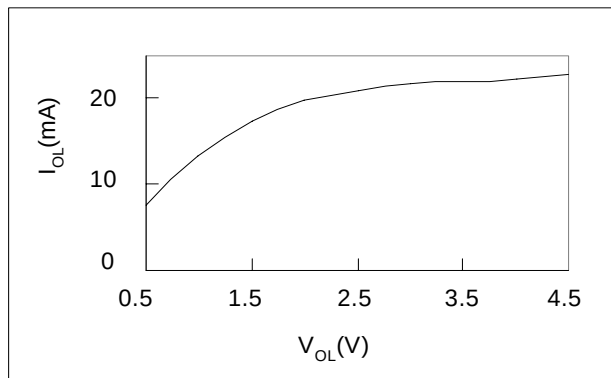
7.11. I/O Output Low Current I_{OL} and V_{OL}
