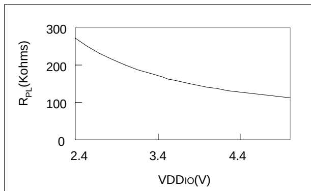
7.10. Pull Low Resister and V_{DDIO}
