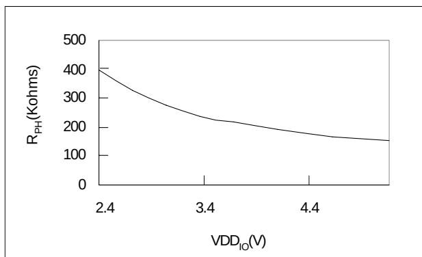
7.8. Pull High Resister and V_{DDIO}
