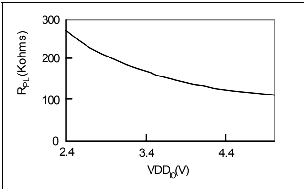
7.10. Pull Low Resistor and VDD IO
