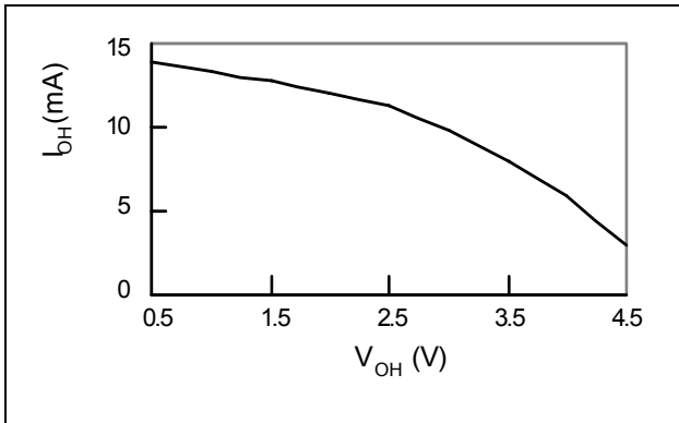
7.9. I/O Output High Current I OH and V OH
