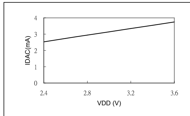
7.13. DAC output current vs. VDD (3mA mode with 500hm resistor)
