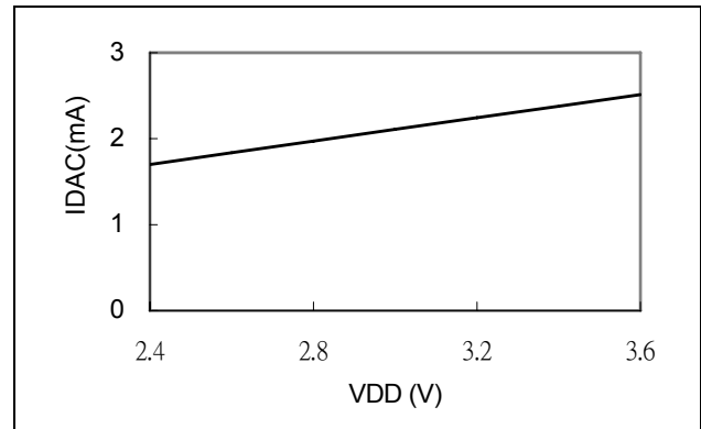
7.12. DAC output current vs. VDD (2mA mode with 500hm resistor)
