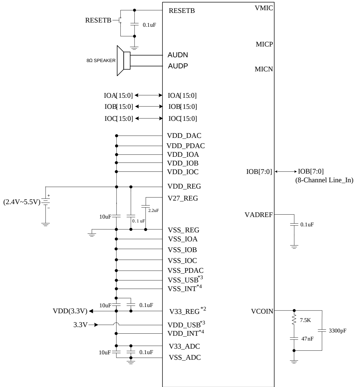
Application Circuit(LINE_IN)
