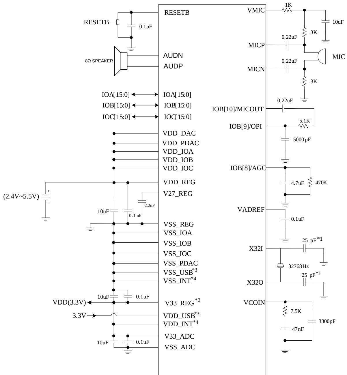
Application Circuit(MIC_IN )
