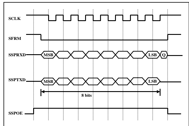
Single transfer Data Change at Rising, Latch at Falling
