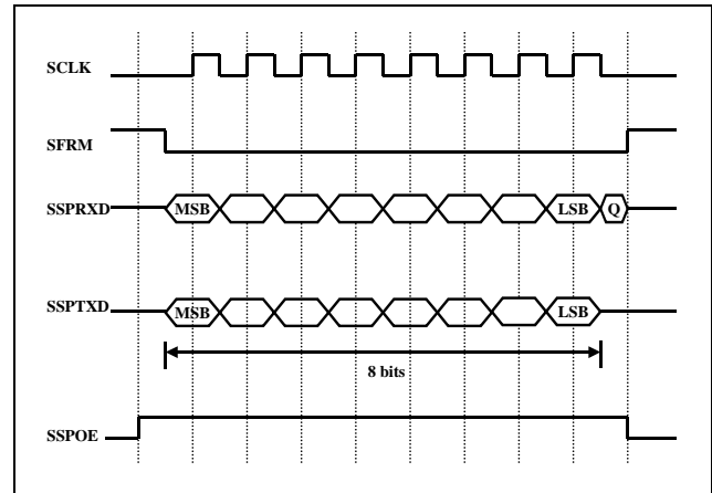
Single transfer Data Change at Falling, Latch at Rising.
