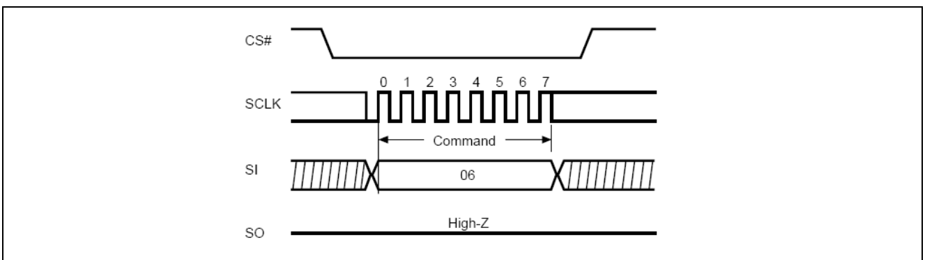
Figure11. Write Enable (WREN) Sequence (Command 06)
