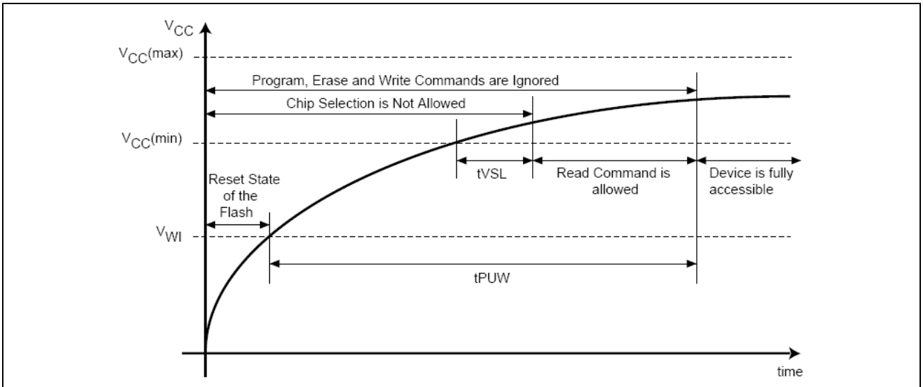
Figure26. Power-up Timing
