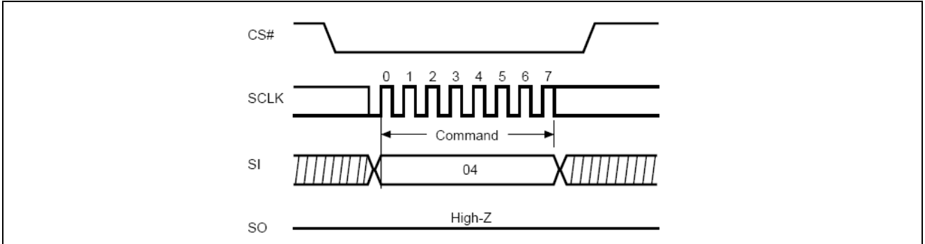
Figure12. Write Disable (WRDI) Sequence (Command 04)
