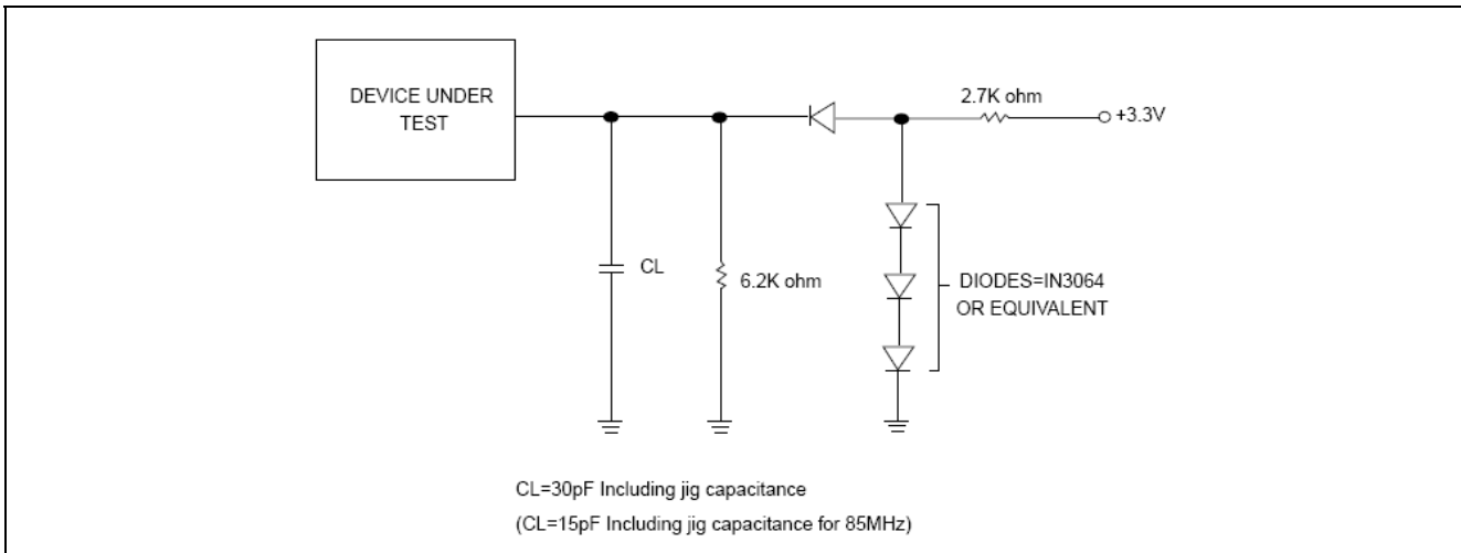
Figure6. Output Loading
