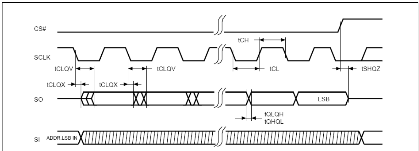
Figure8. Output Timing
