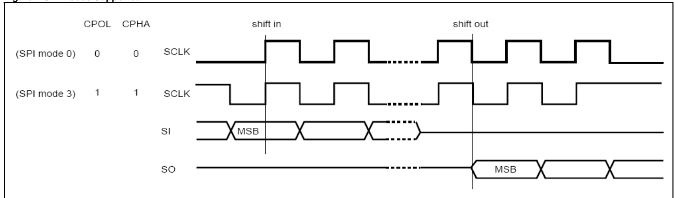
Figure2. SPI Modes Supported
