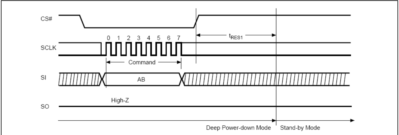
Figure24. Release from Deep Power-down (RDP) Sequence (Command AB)
