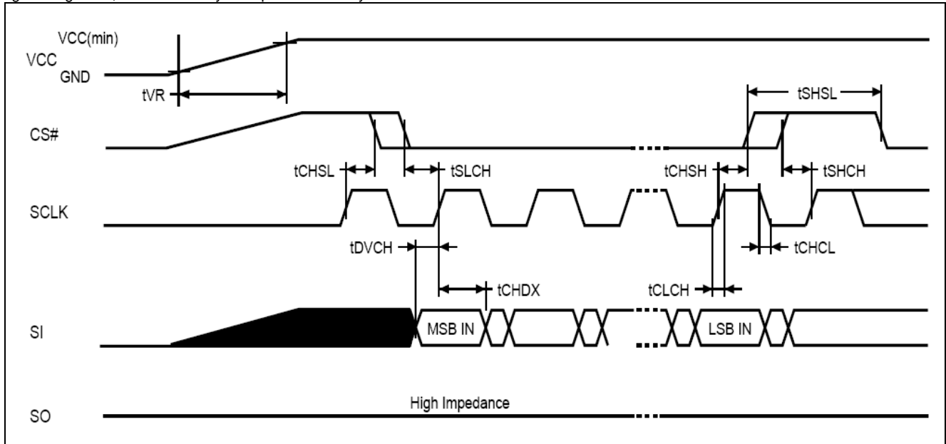
Figure A. AC Timing at Device Power-Up
