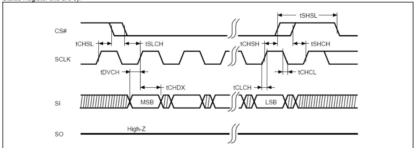
Figure7. Serial Input Timing
