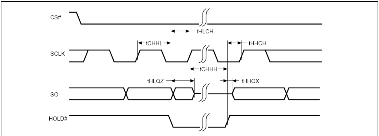
Figure9. Hold Timing
