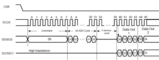
Figure 12. Dual Read Mode Sequence (Command 3B)
