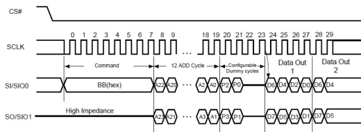
Figure 13. 2 x I/O Read Mode Sequence (Command BB)
