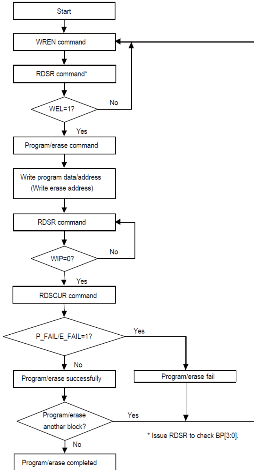
Figure 26. Program/Erase Flow(2) without read array data
