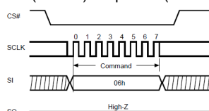
Figure 3. Write Enable (WREN) Sequence (Command 06)
