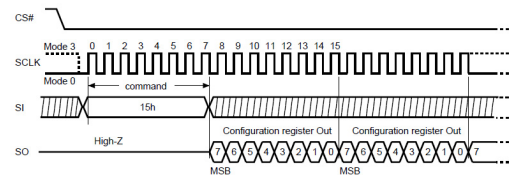
Figure 7. Read Configuration Register (RDCR) Sequence
