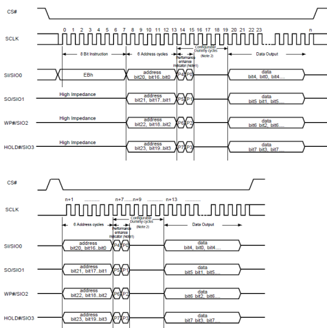
Figure 16. 4 x I/O Read enhance performance Mode Sequence (Command EB) (SPI Mode)
