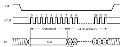
Figure 21. Block Erase 32KB (BE32K) Sequence (Command 52)
