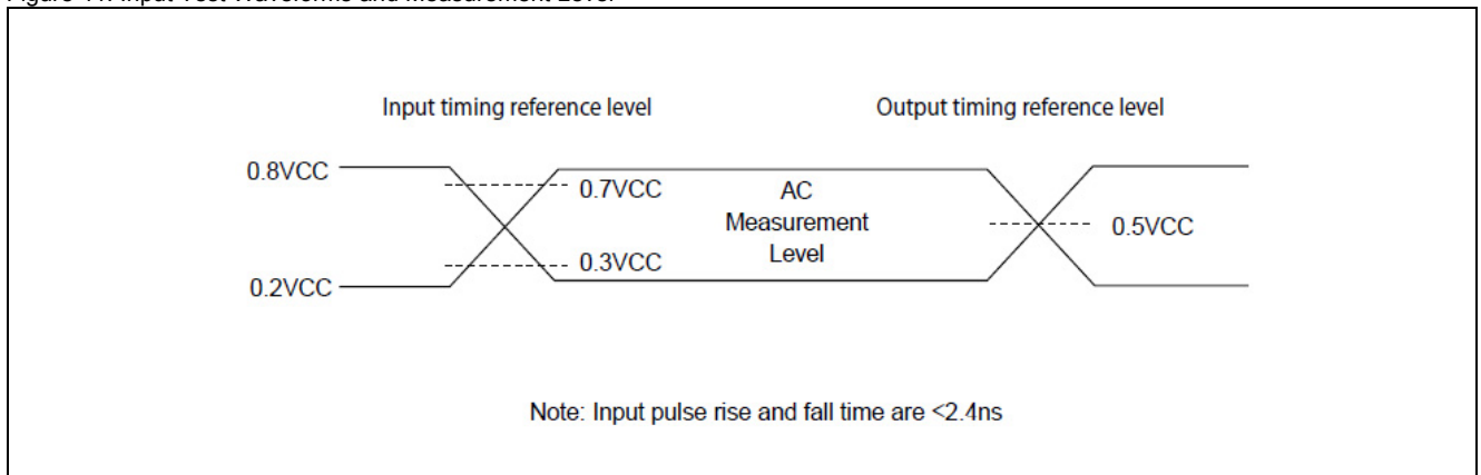
Figure 41. Input Test Waveforms and Measurement Level
