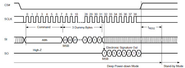
Figure 29. Release from Deep Power-down (RDP) Sequence
