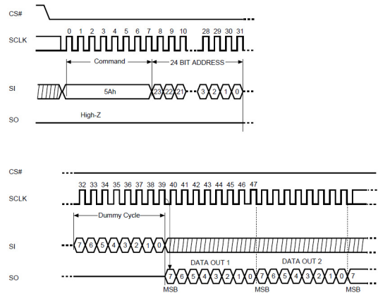
Figure 38. Read Serial Flash Discoverable Parameter (RDSFDP) Sequence
