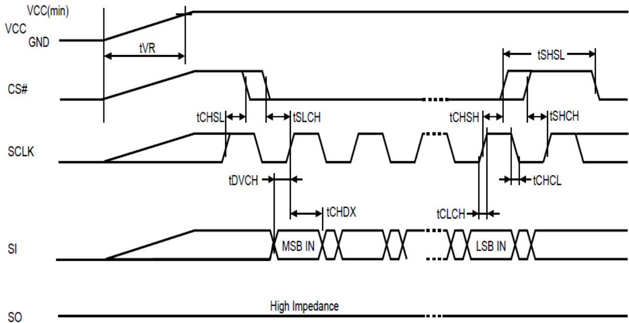
Figure 47. AC Timing at Device Power-Up
