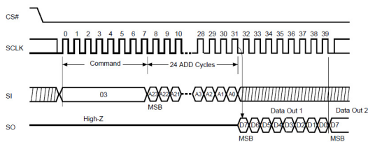
Figure 10. Read Data Bytes (READ) Sequence (Command 03)
