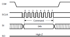
Figure 4. Write Disable (WRDI) Sequence (Command 04)
