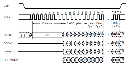
Figure 24. 4 x I/O Page Program (4PP) Sequence (Command 38)
