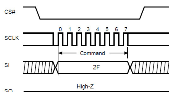
Figure 32. Write Security Register (WRSCUR) Sequence (Command 2F) (SPI mode)
