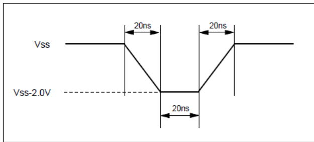
Figure 39. Maximum Negative Overshoot Waveform
