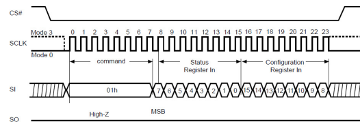
Figure 8. Write Status Register (WRSR) Sequence (Command 01)
