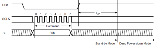
Figure 27. Deep Power-down (DP) Sequence (Command B9)
