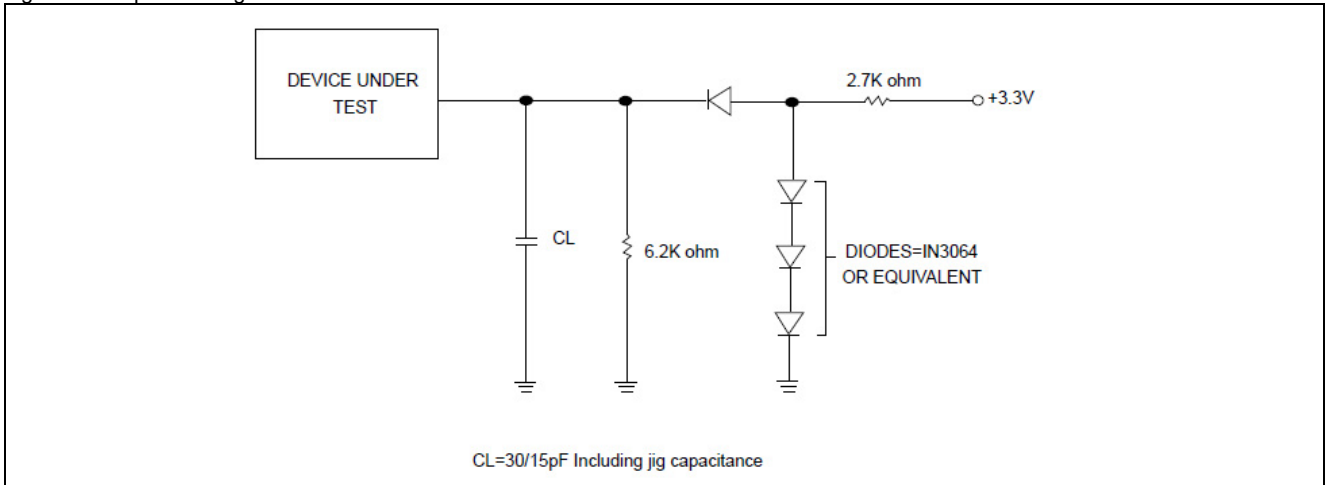
Figure 42. Output Loading
