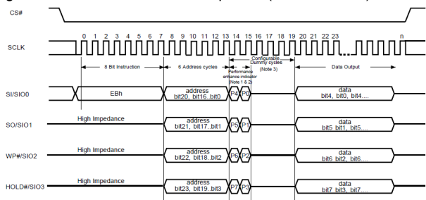
Figure 15. 4 x I/O Read Mode Sequence (Command EB)
