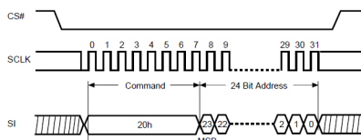
Figure 19. Sector Erase (SE) Sequence (Command 20)
