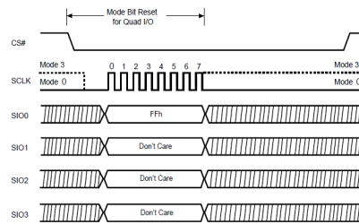
Figure 17. Performance Enhance Mode Reset for Fast Read Quad I/O
