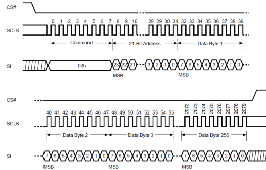
Figure 23. Page Program (PP) Sequence (Command 02)
