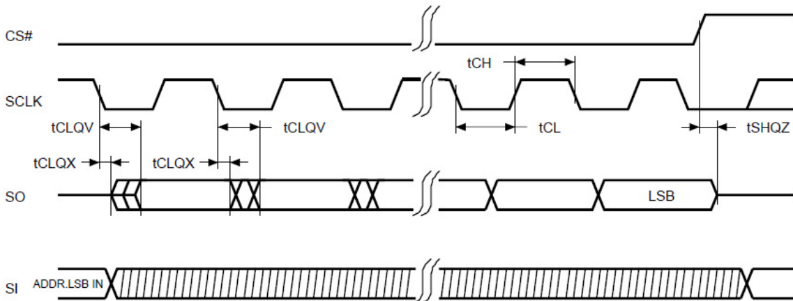
Figure 44. Output Timing
