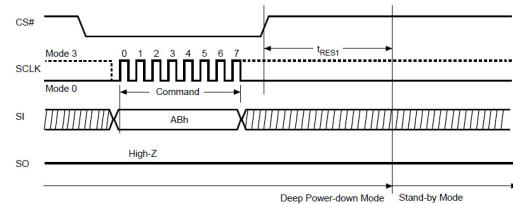
Figure 29. Release from Deep Power-down (RDP) Sequence
