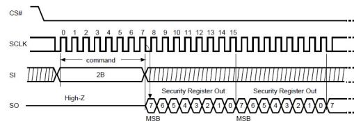
Figure 31. Read Security Register (RDSCUR) Sequence (Command 2B)
