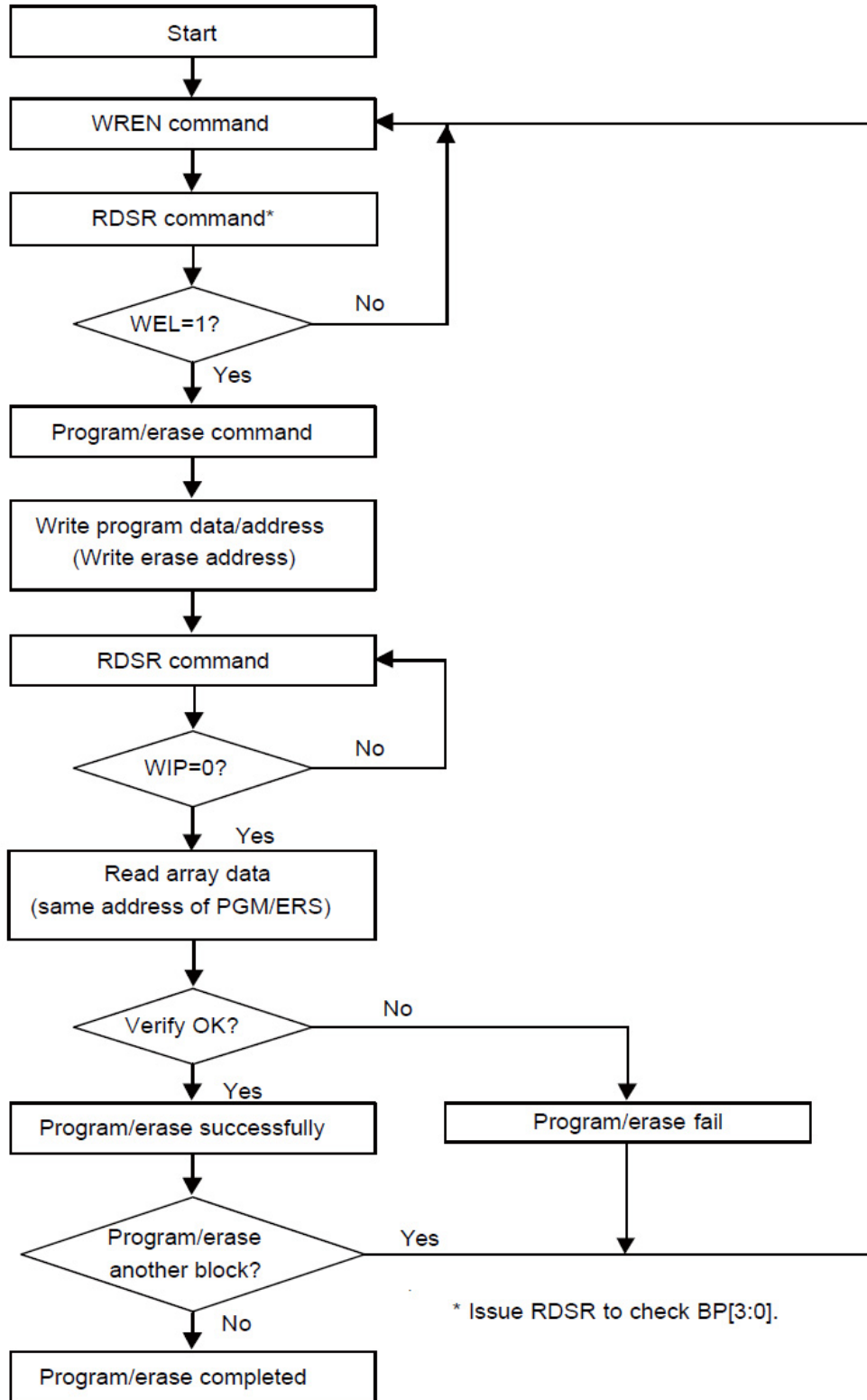
Figure 25. Program/Erase Flow(1) with read array data
