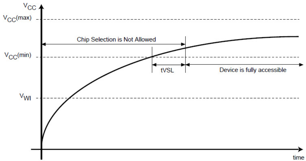
Figure 50. Power Up/Down and Voltage Drop
