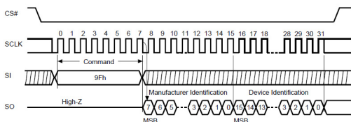
Figure 5. Read Identification (RDID) Sequence (Command 9F)
