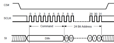
Figure 20. Block Erase (BE) Sequence (Command D8)
