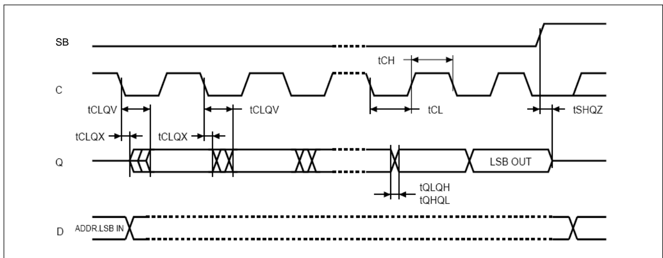
Figure10. Output Timing
