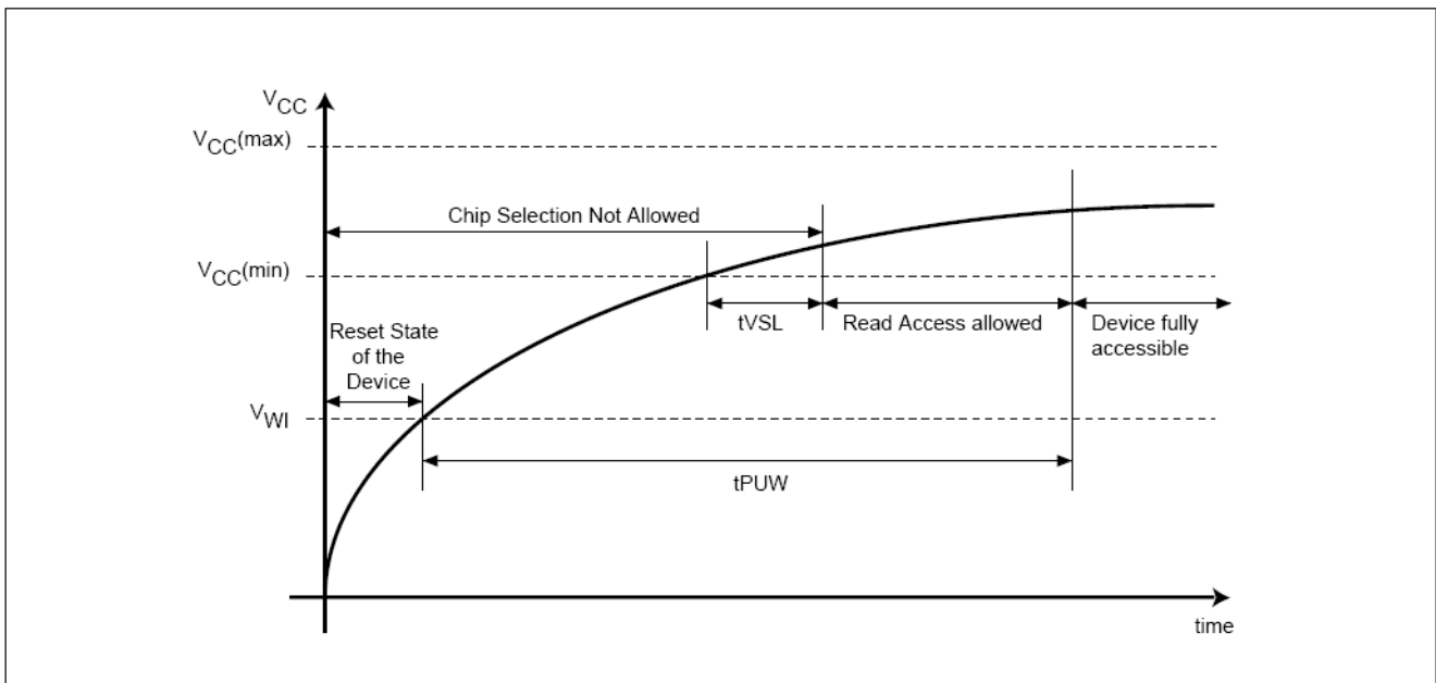
Figure6. Power-up Timing
