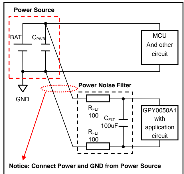
Figure 18. Application Suggestions for reducing power noise
