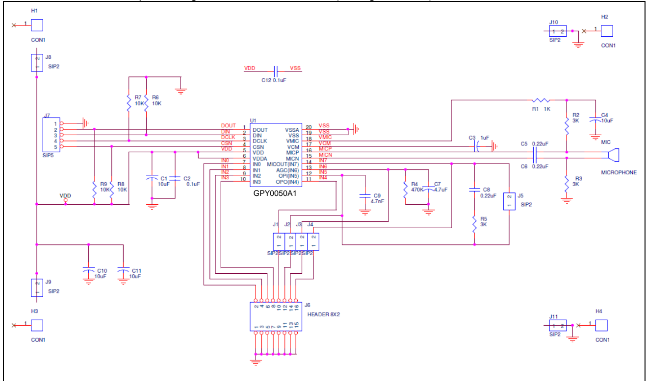
Figure 16. Demo Board Circuit of the GPY0050A1
