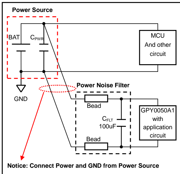
Figure 17. Application Suggestions for Reducing Power Noise
