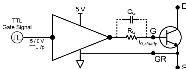
Figure 10: TTL Gate Drive Schematic
