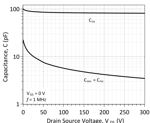
Figure 6: Input, Output, and Reverse Transfer Capacitance
