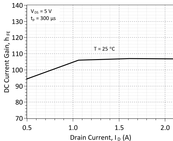
Figure 2: DC Current Gain vs. Drain Current
