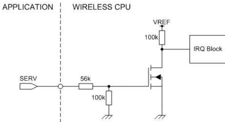
Figure 23: SERVICE Pin Interface
