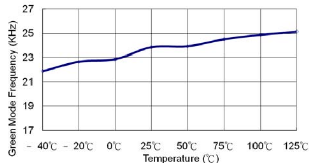
Fig.6 Green Mode Frequency v.s. Temperature
