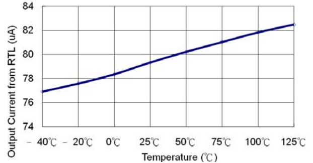
Fig.8 Output Current from RTL v.s. Temperature
