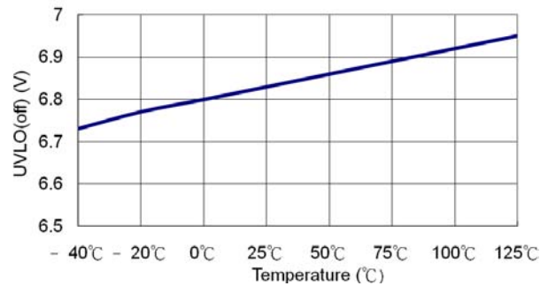
Fig.2 UVLO(off) v.s. Temperature
