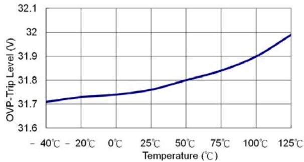
Fig.3 OVP Trip Level v.s. Temperature
