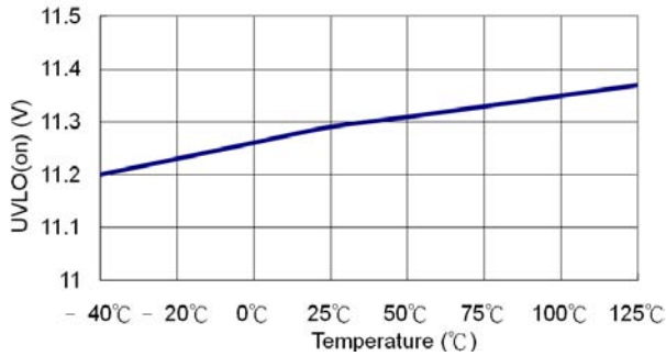
Fig.1 UVLO(on) v.s. Temperature
