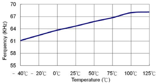
Fig.5 Frequency v.s. Temperature
