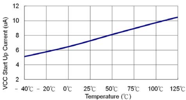
Fig.7 VCC Start Up Current v.s. Temperature
