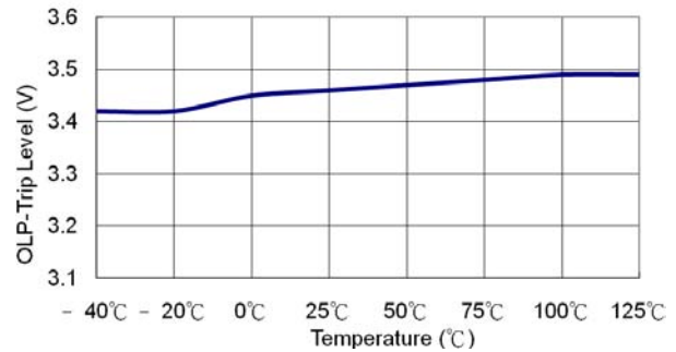
Fig.4 OLP Trip Level v.s. Temperature
