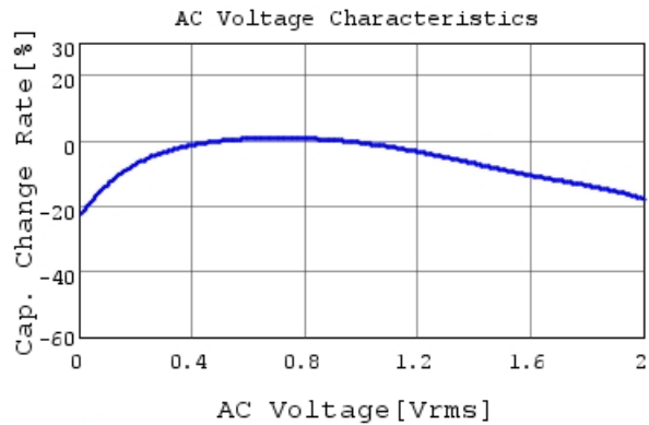
GRM186R60J226ME15 C-AC Voltage capchange, DC
