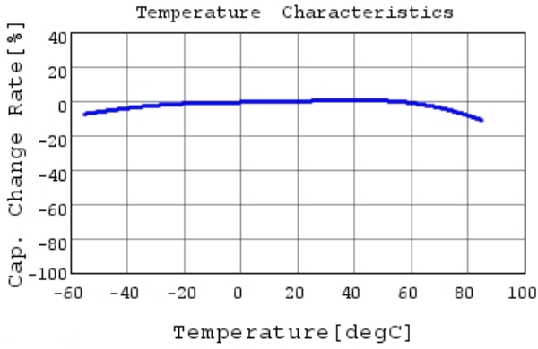
GRM186R60J226ME15 C-Temp. capchange, DC0.0V,
