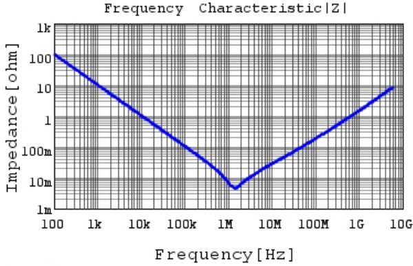
GRM186R60J226ME15 |Z| DCOV, 25degC
