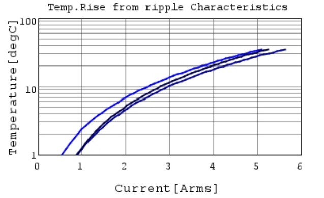
GRM186R60J226ME15 Temp.rise — 80kHz
