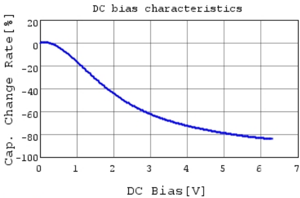
GRM186R60J226ME15 C-DC bias capchange, 25.0c
