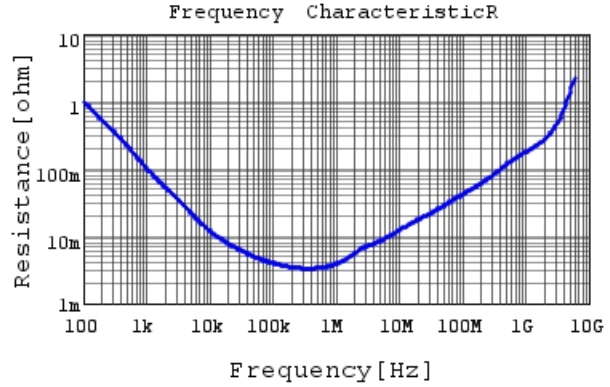
GRM186R60J226ME15 R DCOV, 25degC
