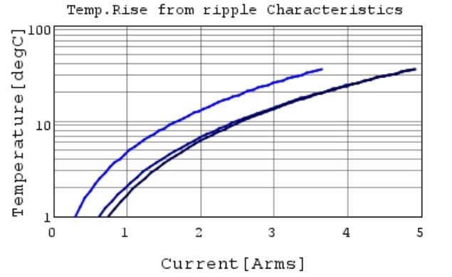
GRM188R61E106MA73 Temp.rise — 80kHz
