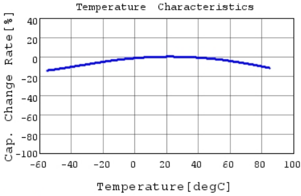
GRM188R61E106MA73 C-Temp. capchange, DC0.0V,
