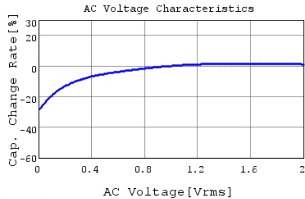
GRM188R61E106MA73 C-AC Voltage capchange, Dc
