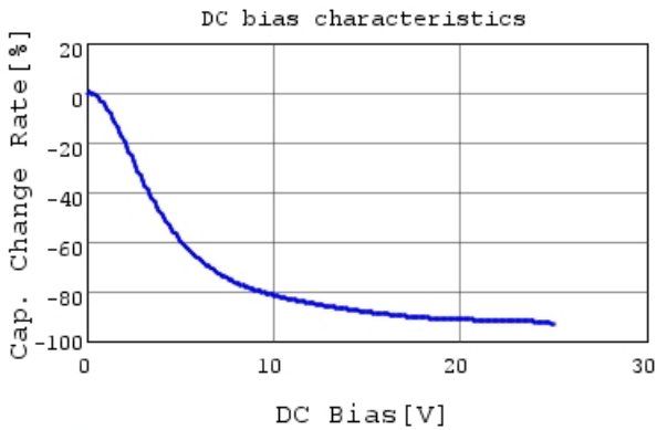
GRM188R61E106MA73 C-DC bias capchange, 25.0c
