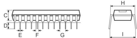
Fig2. 1/2 Lead Packages
