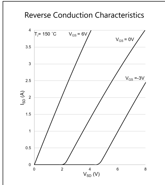
Figure 10: Typical I_{SD} vs. V_{SD} @ T_J = 150\text{ }^\circ\text{C}
