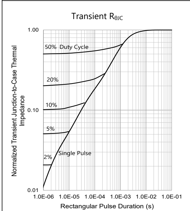
(1.00 = Nominal DC thermal impedance)
