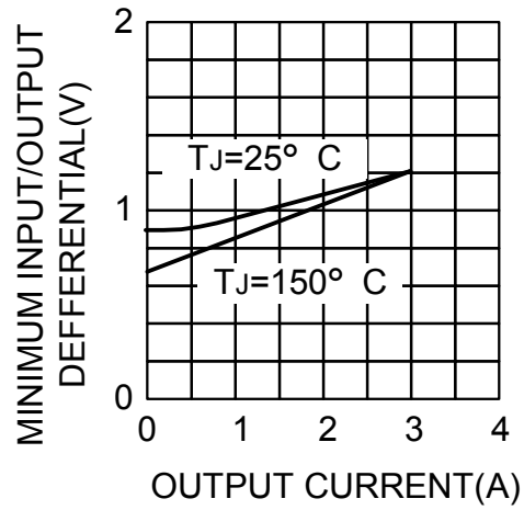
Dropt Voltage
