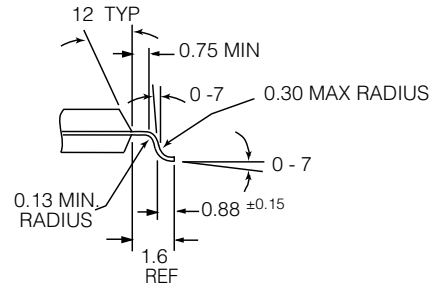
128 pin MQFP
