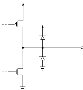
Figure 3-8: Indicator Outputs: SD/HD, LD
