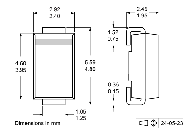
Fig. 12. Package outline SMA (SOD1001-1)
