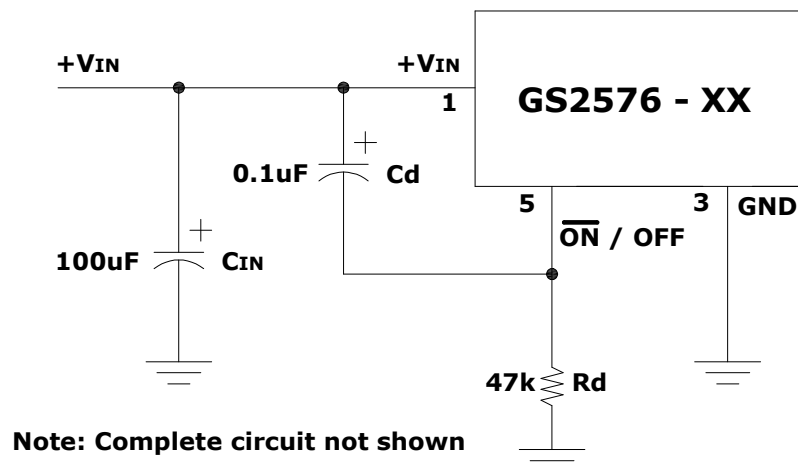
FIGURE 6. Delayed Startup
