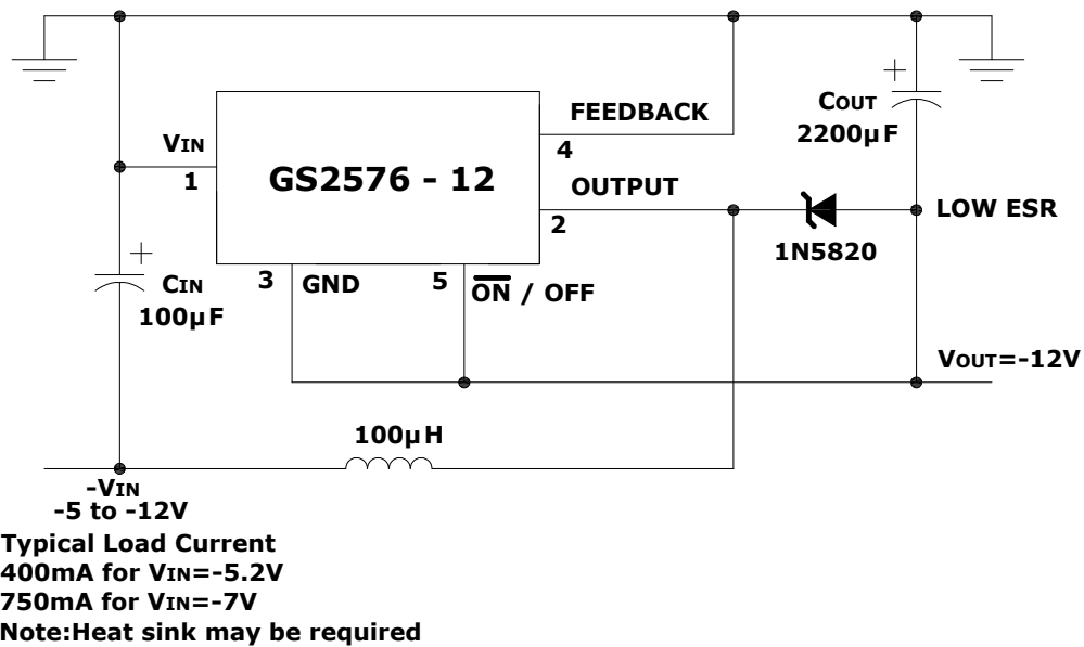
FIGURE 3. Negative Boost
