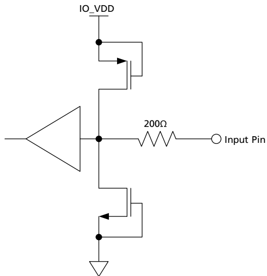
Figure 3-2: Digital Input Pin (20bit/10bit, \overline{\text{ANC\_BLANK}} , \overline{\text{DETECT\_TRS}} , DVB_ASI, RATE_SEL0, \overline{\text{SMPTE\_BYPASS}} , RATE_SEL1, TIM_861, F/DE, H/HSYNC, PCLK, V/VSNC)
