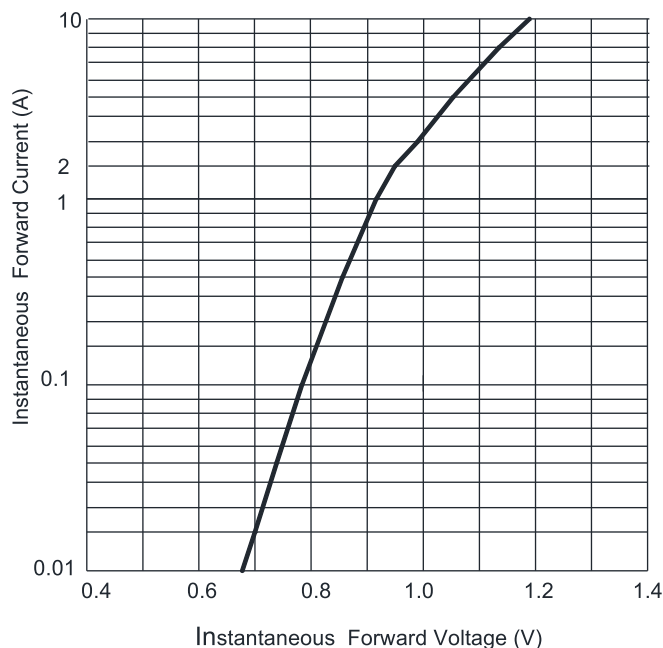
FIG3: Forward Voltage
