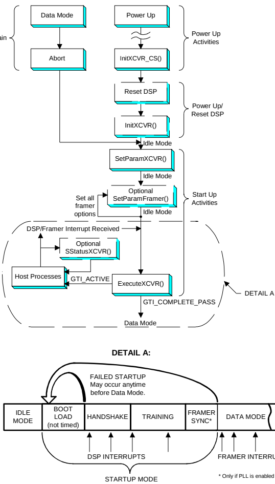
Figure 2. Typical Transceiver Power Up/Start Up Sequence
