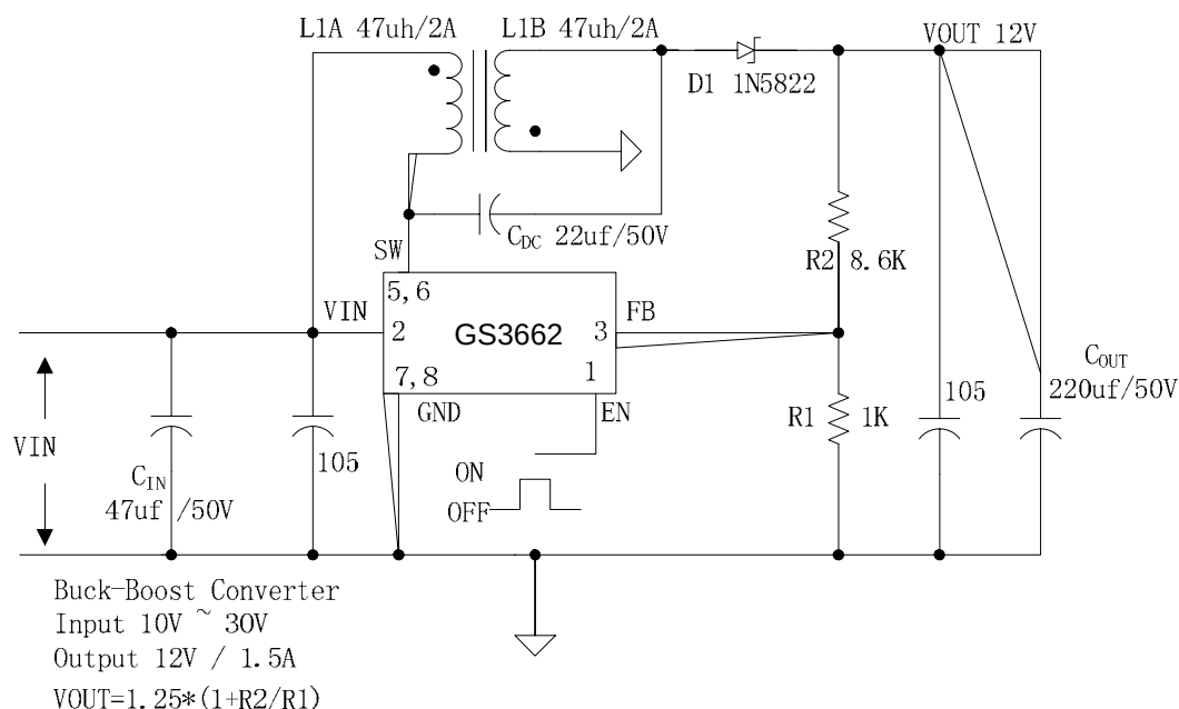
Figure6. GS3662 Typical System Application (SEPIC Buck-Boost Converter)
