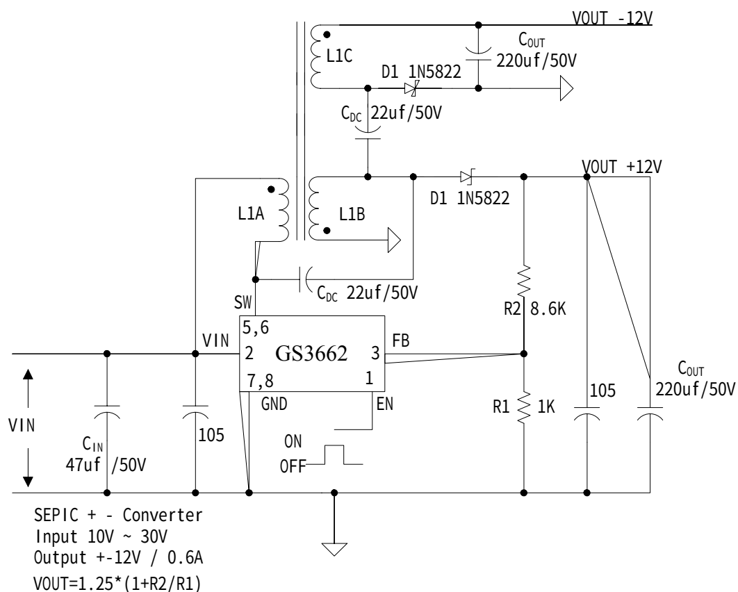
Figure8. GS3662 Typical System Application (SEPIC Inverting Converter)
