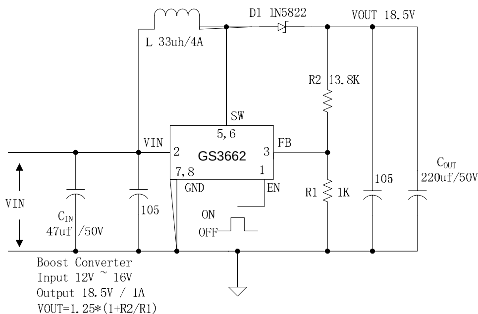
Figure5. GS3662 Typical System Application (Boost Converter)
