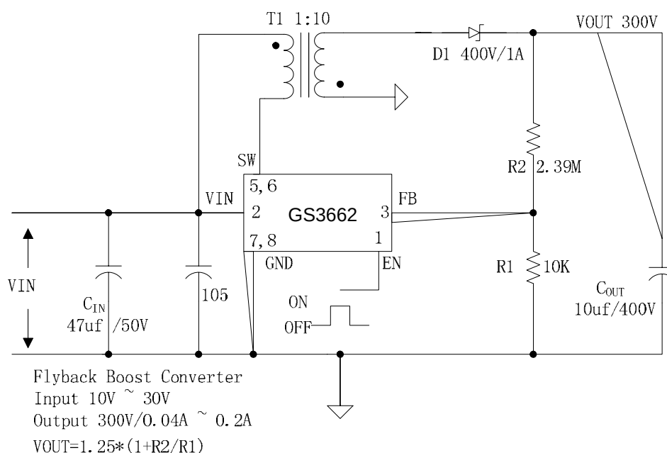
Figure7. GS3662 Typical System Application (Flyback Boost Converter)
