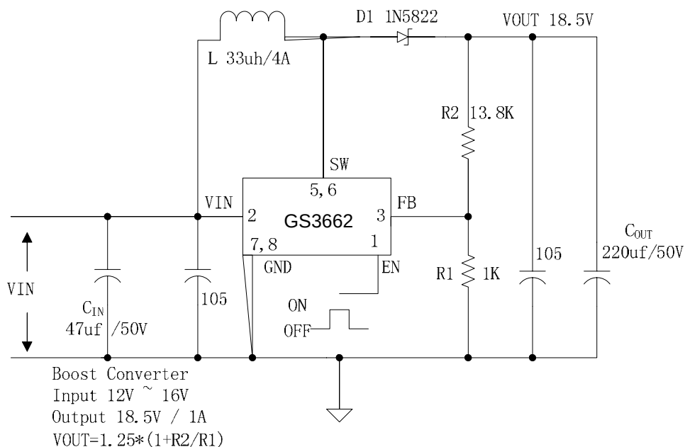
Figure4. GS3662 Typical Application Circuit (Boost Converter)
