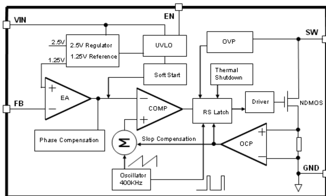
Figure3. Function Block Diagram of GS3662
