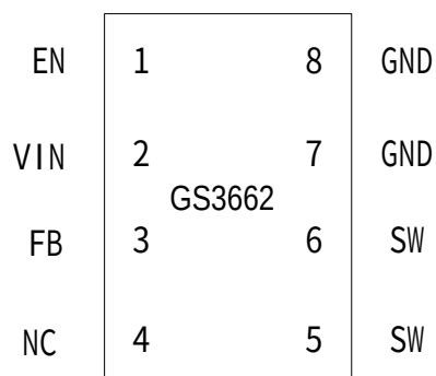
Figure2. Pin Configuration of GS3662 (Top View)
