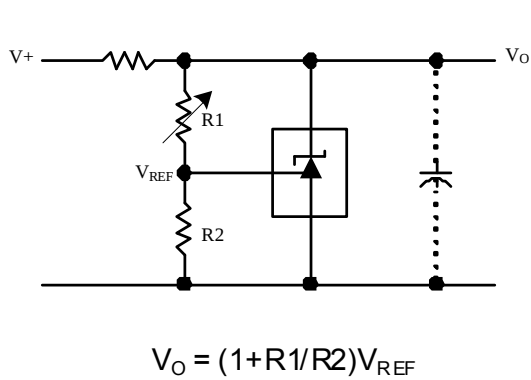
Shunt Regulator
