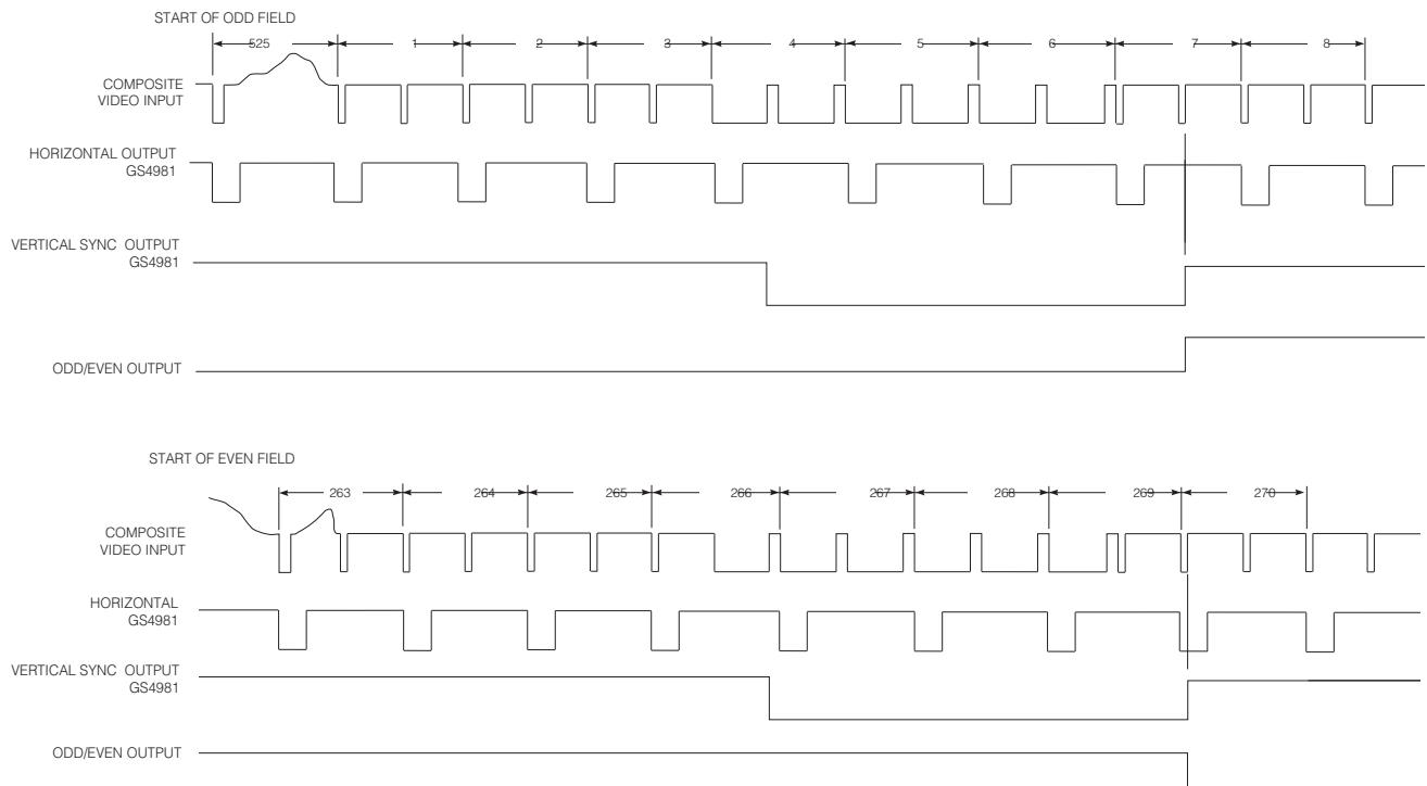
Figure 5-11: Timing Diagram
