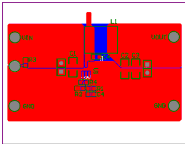
Figure 3. GS5470 Suggested Layout
