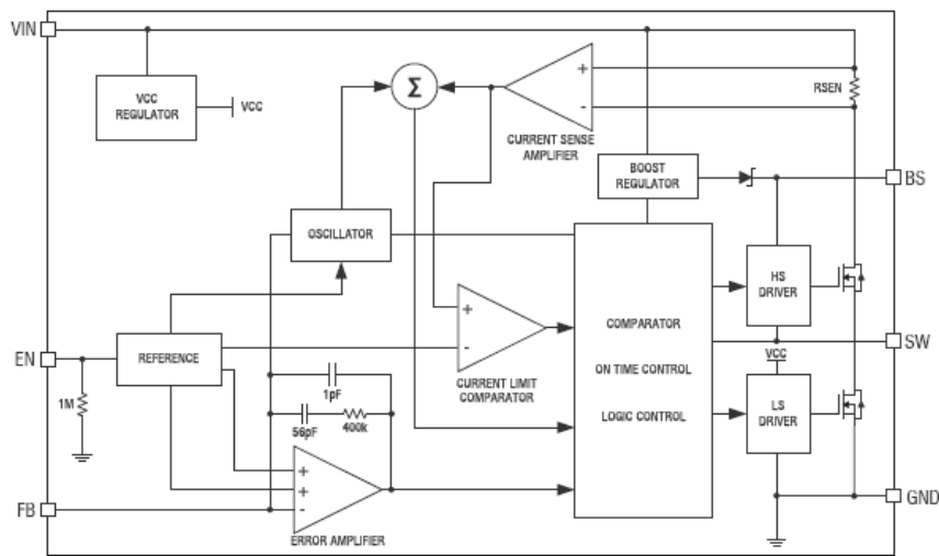
Figure 2. GS5470 Block Diagram
