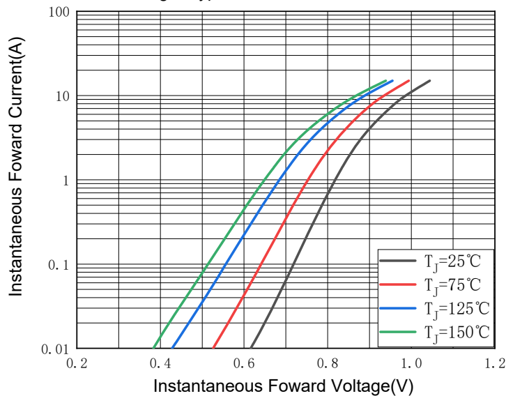
Fig 3:Typical Foward Characteristics
