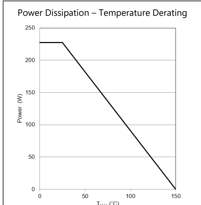
Figure 14: Power Derating vs. T_{case}
