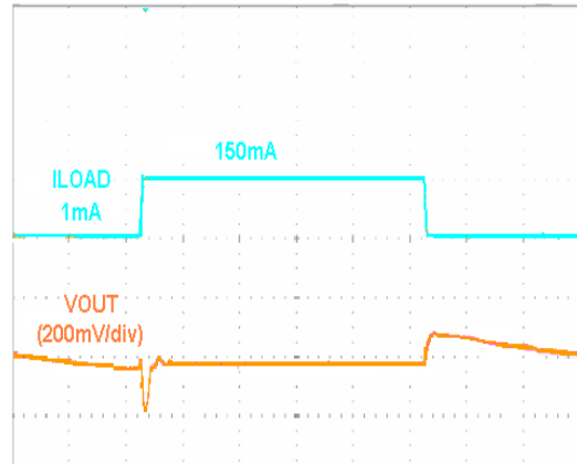
Time (10us/div)
