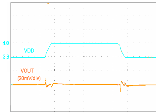
Time (10us/div)
