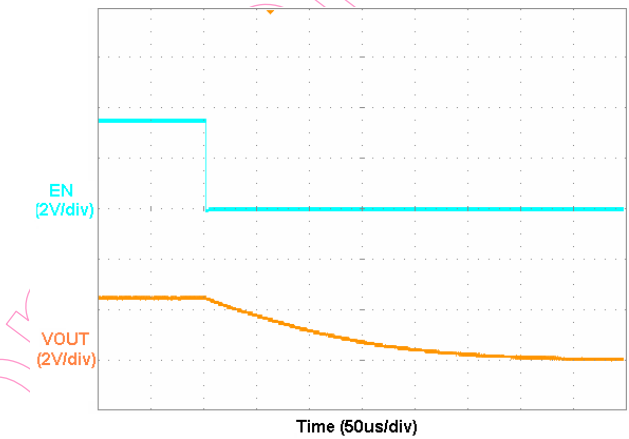
V_{OUT}=2.5V, I_{OUT}=0mA, V_{DD}=3.5V
