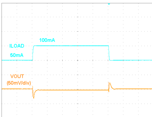
Time (10us/div)
