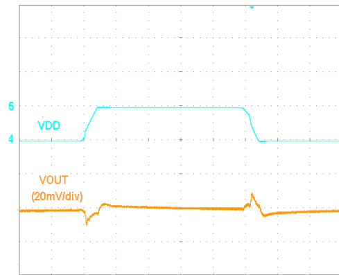
Time (10us/div)
