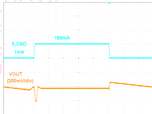
Time (10us/div)
