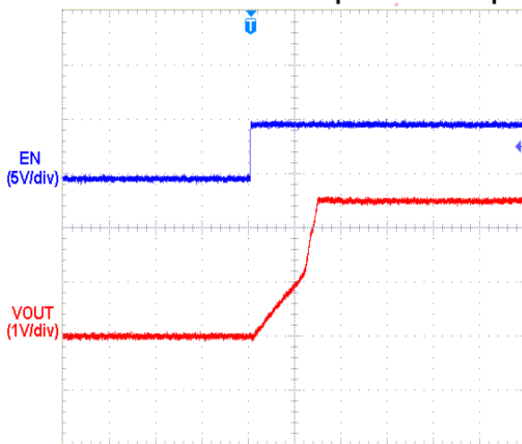
V_{OUT}=2.5V , I_{OUT}=0mA , V_{DD}=3.5V
