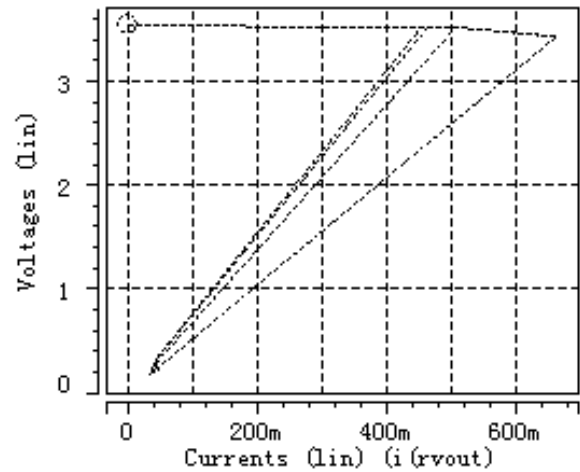
Output Voltage vs. Output Current ( C_{in}=1.0\mu F, C_{out}=1.0\mu F, Temp=25^{\circ}C )
