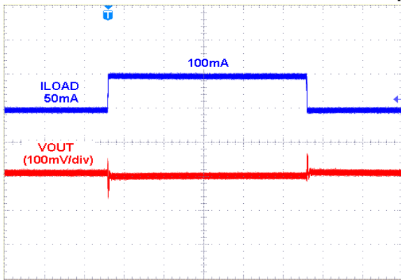
V_{OUT}=2.5V , I_{OUT}=50mA \sim 100mA \sim 50mA , V_{DD}=3.5V tr=tf=0.5\mu s
