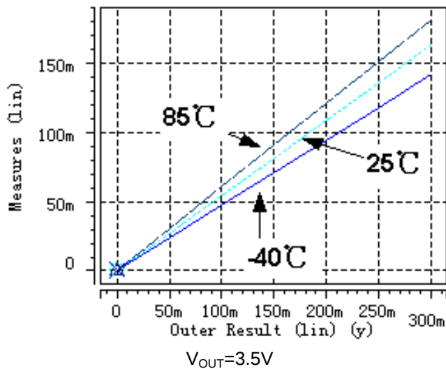
Dropout Voltage vs. Output Current (Cin=1.0uF, Cout=1.0uF)
