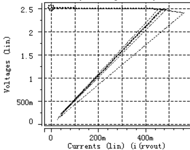
Output Voltage vs. Output Current ( C_{in}=1.0\mu F, C_{out}=1.0\mu F, Temp=25^{\circ}C )
