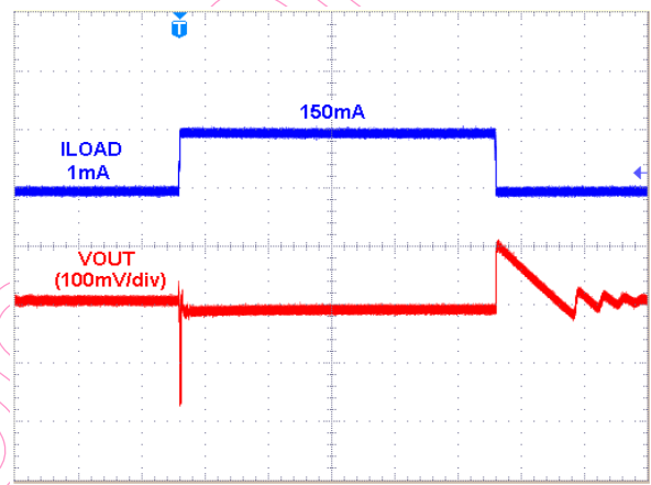
V_{OUT}=3.0V , I_{OUT}=1mA \sim 150mA \sim 1mA , V_{DD}=4.0V tr=tf=0.5\mu s
