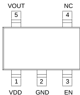
Figure 3c SOT-23-5 /SOT-353 Package
