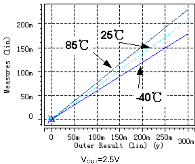
Dropout Voltage vs. Output Current (Cin=1.0uF, Cout=1.0uF)
