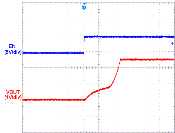
V_{OUT}=2.5V , I_{OUT}=150mA , V_{DD}=3.5V
