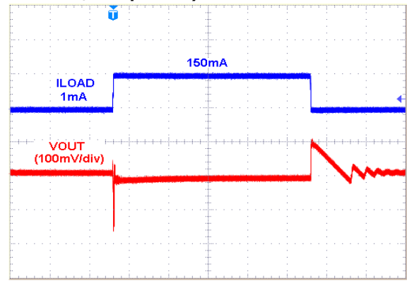
V_{OUT}=2.5V , I_{OUT}=1mA \sim 150mA \sim 1mA , V_{DD}=3.5V tr=tf=0.5\mu s
