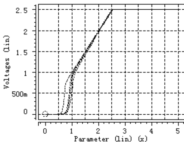
Output Voltage vs. Input Voltage ( C_{in}=1.0\mu F, C_{out}=1.0\mu F, Temp=25^{\circ}C )
