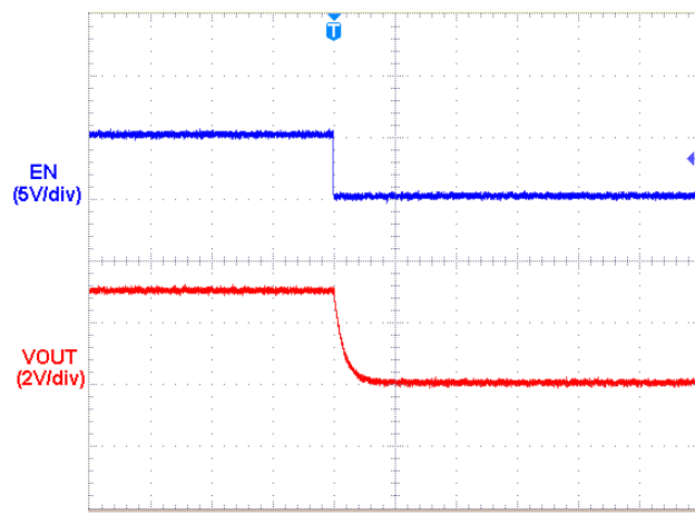
Time(100us/div) V_{OUT}=3.0V , I_{OUT}=150mA , V_{DD}=4.0V
