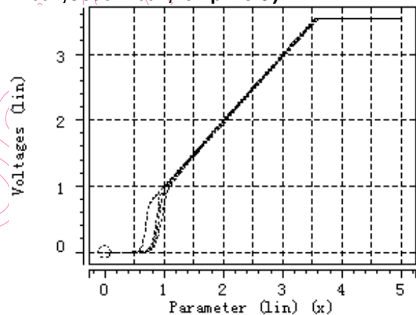
Output Voltage vs. Input Voltage ( C_{in}=1.0\mu F, C_{out}=1.0\mu F, Temp=25^{\circ}C )
