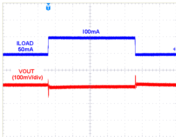
V_{OUT}=3.0V , I_{OUT}=50mA \sim 100mA \sim 50mA , V_{DD}=4.0V tr=tf=0.5\mu s
