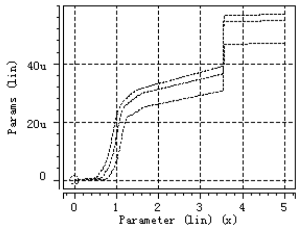
Supply Current vs. Input Voltage ( C_{in}=1.0\mu F, C_{out}=1.0\mu F, Temp=25^{\circ}C )
