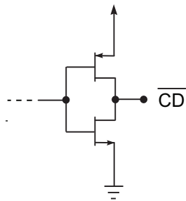
Figure 5-5: \overline{CD} Circuit
