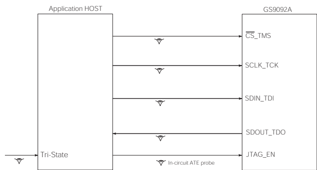
Figure 3-18: System JTAG
