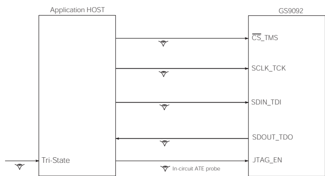
Figure 3-16: System JTAG
