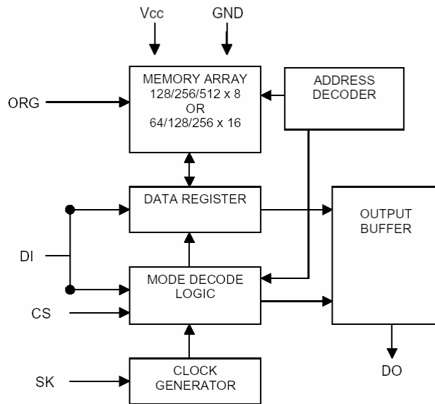
Figure 2. Block Diagram
