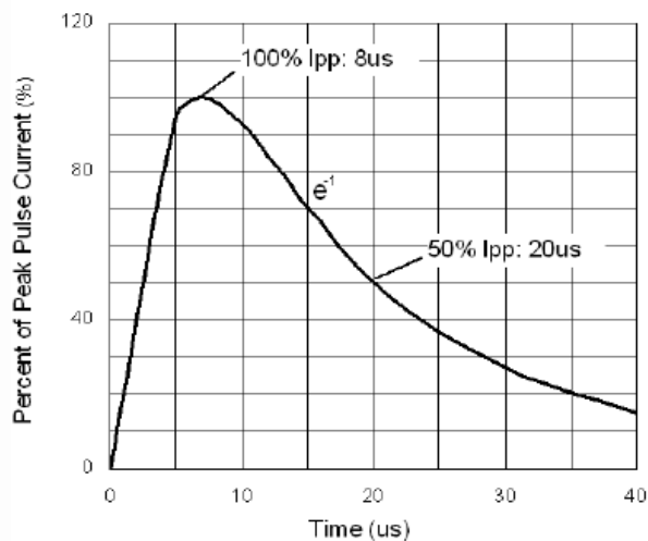
Figure 1. 8/20 \mu s pulse waveform according to IEC 61000-4-5
