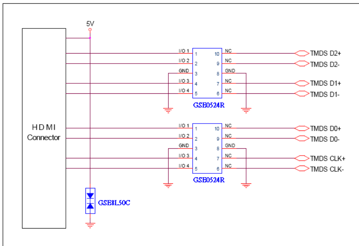
HDMI Interface ESD Protection
