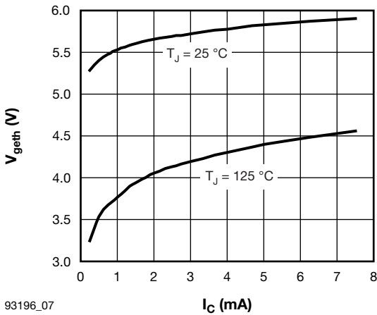
Fig. 7 - Typical IGBT Threshold Voltage
