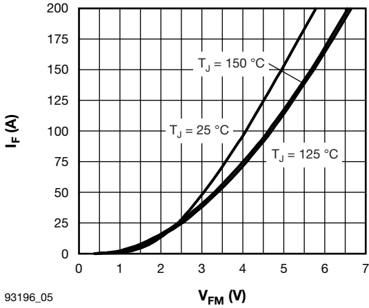
Fig. 5 - Typical Diode Forward Characteristics
