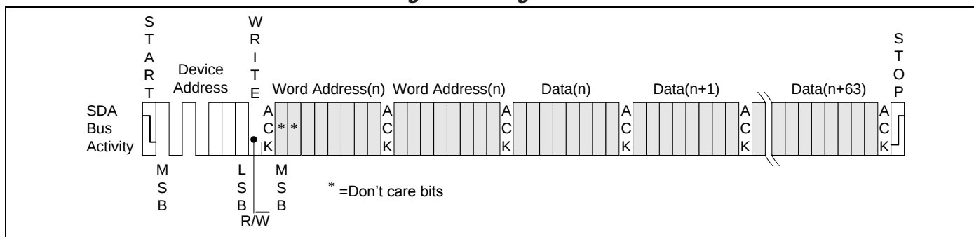
Figure 5-7. Page Write
