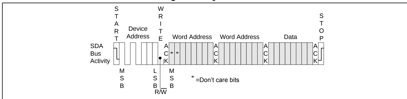
Figure 5-6. Byte Write
