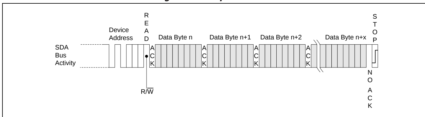
Figure 5-10. Sequential Read
