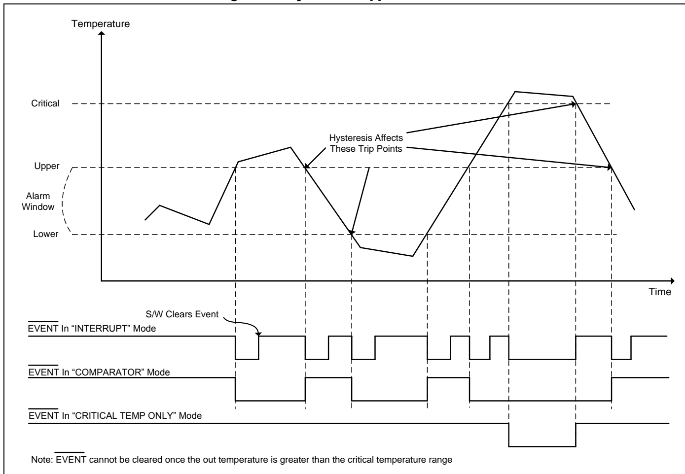
Figure 6.2 Hysteresis Applied Condition
