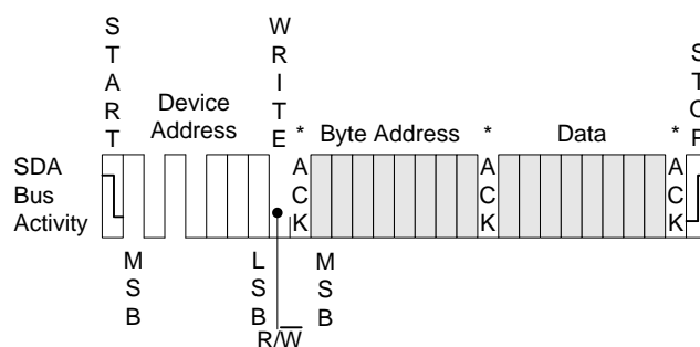
Figure 7.2 Byte Write
