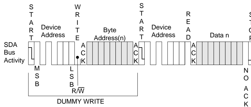
Figure 7.5 Random Address Read
