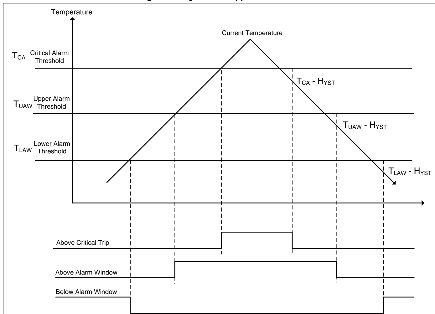
Figure 6.1 Hysteresis Applied Condition
