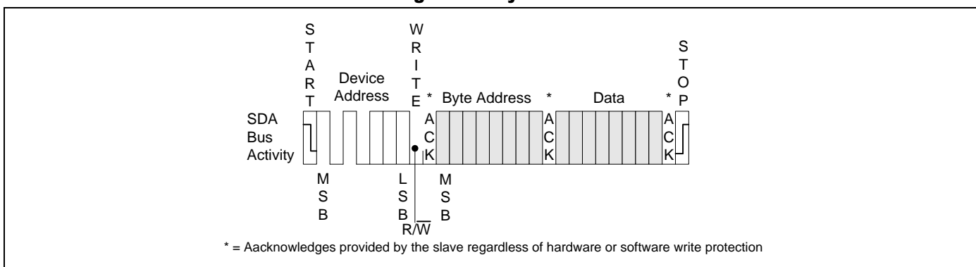
Figure 7.2 Byte Write
