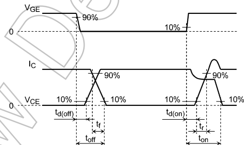
Fig. 6.2.2 Timing Chart of Switching Time
