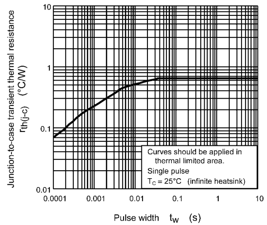
Fig. 8.10 r_{th(j-c)} - t_w (Guaranteed Maximum)
