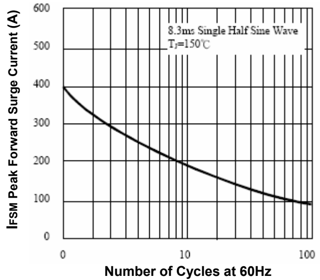
Fig.2- Max. Non-Repetitive Forward Surge Current
