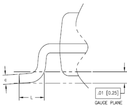
DETAIL F ROTATED 90° CCW SCALE: 30/1
