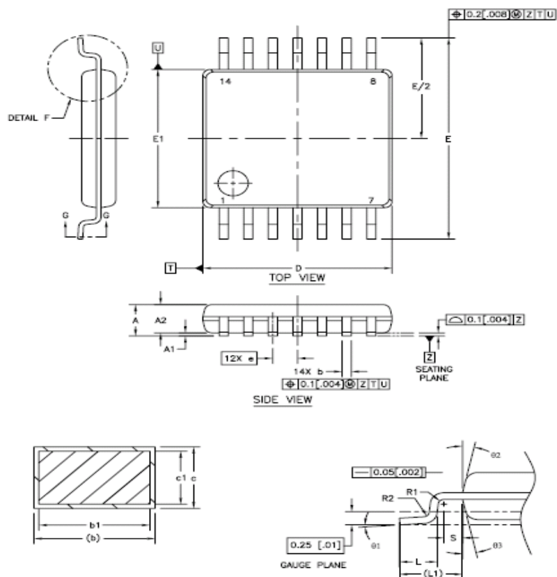
DETAIL F ROTATED 90° CCW SCALE: 20/1
