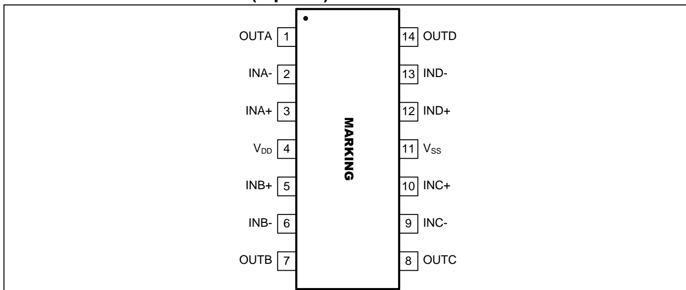
Figure 1. Pin Assignment Diagram (SOP14 and TSSOP14 Package)
