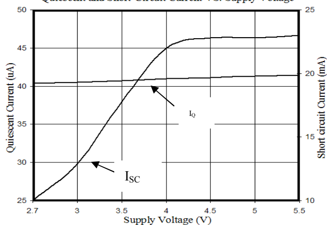
Quiescent and Short-Circuit Current VS. Supply Voltage
