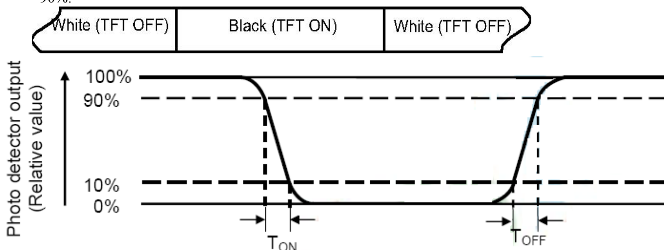
Fig. 4-3 Definition of response time
