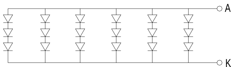
LED Circuit
