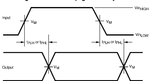
Voltage Waveform - Propagation Delay Times
