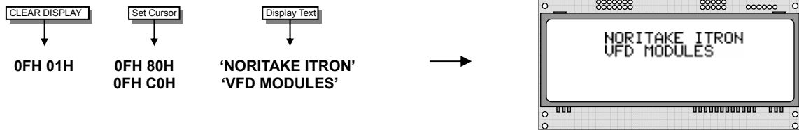
Displaying text using Serial Communications
